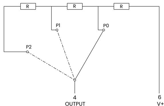
CIRCUIT DIAGRAM FOR SHUNT RESISTOR OUTPUT
