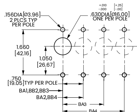
PANEL CUTOUT DETAIL
