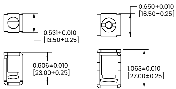
RCT-01 FOR 2 POLE BUSBAR
