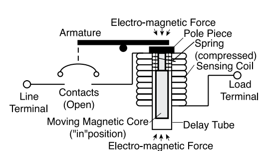
Figure 3 - Moderate Overload with Induced Delay
