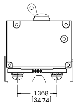
BACK CONNECT SCREW TERMINAL WITH RETAINER -ALTERNATIVE 1.368" SPACING
