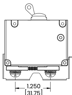
BACK CONNECT SCREW TERMINAL WITH RETAINER
