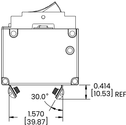
SCREW TERMINAL WITH 30° BEND
