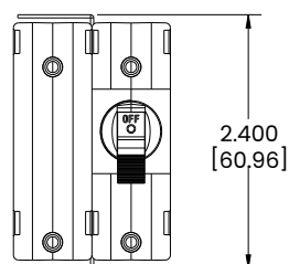
J SERIES CIRCUIT BREAKER WITH 1.250" TERMINAL SPACING AND Z-FOLD TERMINAL BARRIER
